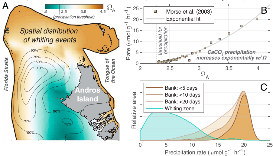
Fig. 4. An exploration of carbonate saturation state and precipitation kinetics in the whitening zone. (A) Aragonite saturation state, based on the water chemistry data from Broecker and Takahashi (30), and whitening occurrence data (32). The 90% contour encapsulates 90% of documented whittings. (B) Carbonate precipitation kinetics based on experiments with Bahama Bank sediment [Morse et al. (47)]. (C) Estimated precipitation rates for different regions of the banktop based on the spatial distribution of \Omega_A (A) and the experimental kinetics data in B. Note that waters along the bank margins—represented here as the regions with banktop water ages less than 5, 10, and 20 days—support precipitation rates that are 3 to 4× larger than waters within the whitening zone.
